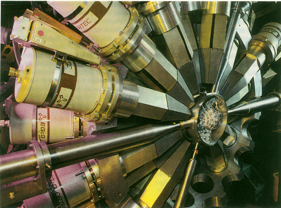
Fig. 3. An overview of one hemisphere of the Gammasphere with the Microball in place. The beam enters from the left.
