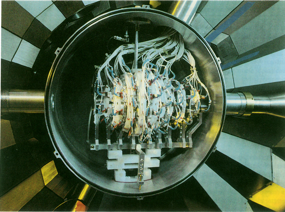
Fig. 2. Close-up photograph of the Microball installed in Gammasphere. The Microball detectors are supported by thin Delrin rings which are held by aluminum legs. The supporting structure allowing 9 degrees of freedom (rotations and translations) is used to align the device to the chamber and the beam axis. The detectors are held by rectangular blocks that hold the two leads of the photodiode. The signal cables are thin shielded coaxial cables ( 75 \Omega ) with teflon insulation and connect the diodes to their preamplifiers located outside the vacuum. Ring 6 is located at exactly 90^\circ and it has an opening to allow the target rod to be inserted in position.
