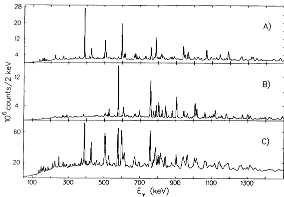
Fig. 11. (a) Low energy part of the spectrum of the \gamma rays from the \alpha 2p exit channel gated by the Microball from the reaction of 130 MeV ^{28}\text{Si} on ^{58}\text{Ni} . (b) Same as in (a) but for the 4p gate. (c) Spectrum from the same reaction but without any particle gating.
