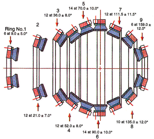
Fig. 1. Schematic diagram showing a vertical section of the Microball. The number of detectors for each ring is indicated. The azimuthal angle \theta and the half angle are also given. The detectors are shown in black facing the target, the light guides are shown as blue trapezoids, the diodes are shown in green, and the supporting Delrin rings in shaded red. The detectors are shown attached to the rings via the gold plated pins (red lines) of the photodiodes.
